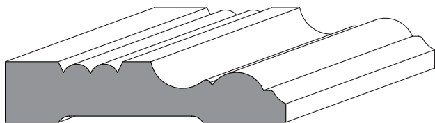
T1-121 3/4 x 3-1/2
