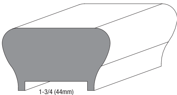
T5-122 1-3/4 x 3
