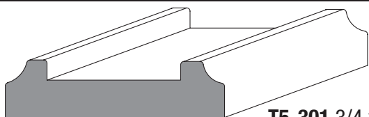
T5-301 3/4 x 2-7/8
