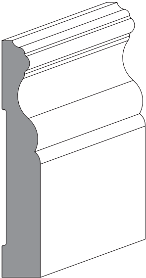
T2-101 11/16 x 4-1/4
