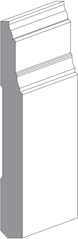
T2-109 11/16 x 7-1/4
