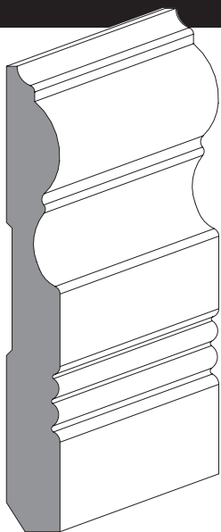
T2-121 11/16 x 5-1/2
