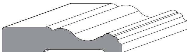
T1-102 3/4 x 3-1/2
